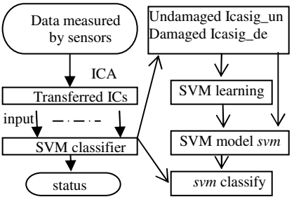
Fig. 2. Frame of integrating ICA and SVM
