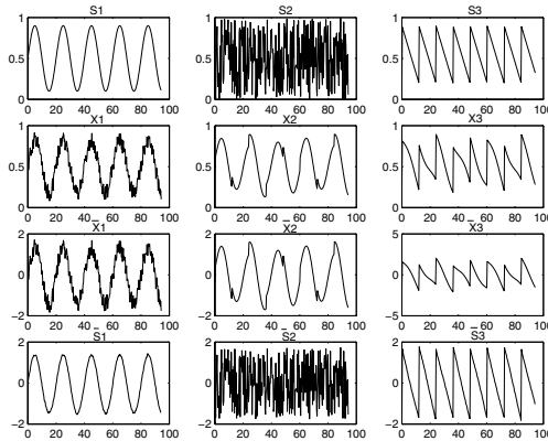
Fig. 1. Clustering Time Series with Noises
