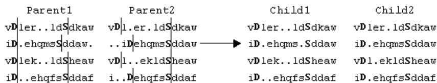
Fig. 3. Two-point crossover
