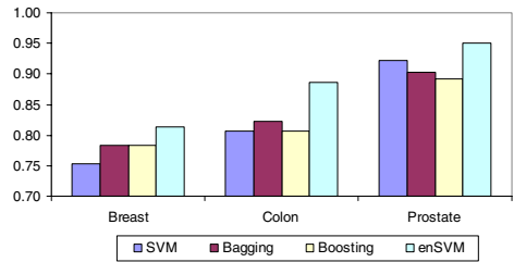
Fig. 5. Classification Accuracies
