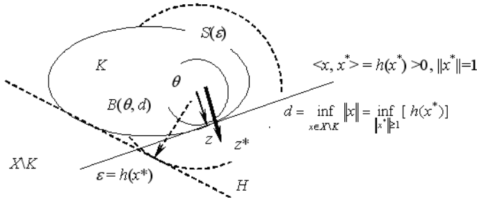
Fig. 2. The distance from the origin \theta to set X \setminus K . Theorem 2 can be geometrically explained as follows: \inf_{\|x^*\| \geq 1} [h(x^*)] = \inf_{\|x^*\| \geq 1} [\sup_{x \in K} \langle x, x^* \rangle] . If x = z , x^* = z^* , \inf_{\|x^*\| \geq 1} [\|x\| \|x^*\|] = \inf_{\|z^*\| \geq 1} [\|z\| \|z^*\|] = \|z\| \|z^*\|_{\|z^*\|=1} = \|z\| . Therefore, we have d = \inf_{x \in X \setminus K} \|x\| = \|z\| = \inf_{\|x^*\| \geq 1} [h(x^*)] , and the alignment of z and z^* .
