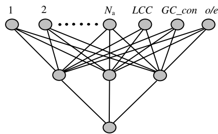
Fig. 2. Promoter_Classifier
