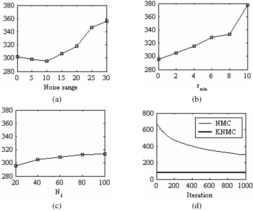
Fig. 2. Comparison of different parameters
