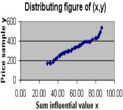
Fig. 5. Distributing figure
