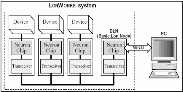
Fig. 3. Connection diagram between LonWorks and internet server using BLN
