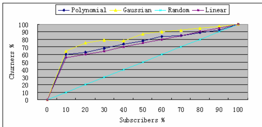
Fig. 1. Lift curve of different kernel function (Polynomial, Gaussian and Linear)
