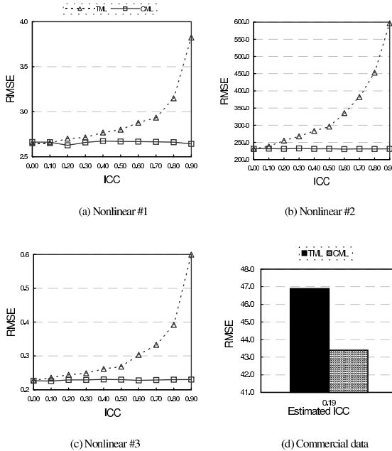
Fig. 3. Global prediction errors
