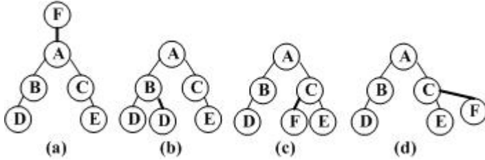
Fig. 4. For a frequent free subtree t , t \setminus v is at location of case (a), (b), or (c), neither t nor any supertree of t correspond to closed or maximal frequent subtrees
