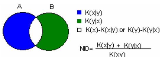
Fig. 1. Illustration of normalized information distance. Circle A is K(x) , circle B is K(y) and the total area of two circles is K(xy)
