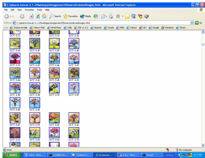
Fig. 4. Experiment 2
