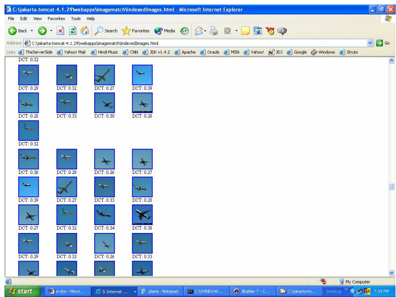
Fig. 3. Experiment 1
