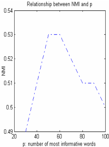
Fig. 3. Relation between NMI and p
