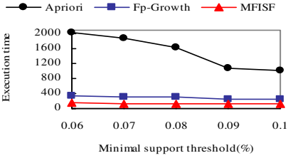
Fig. 4. The performance of algorithms (b)
