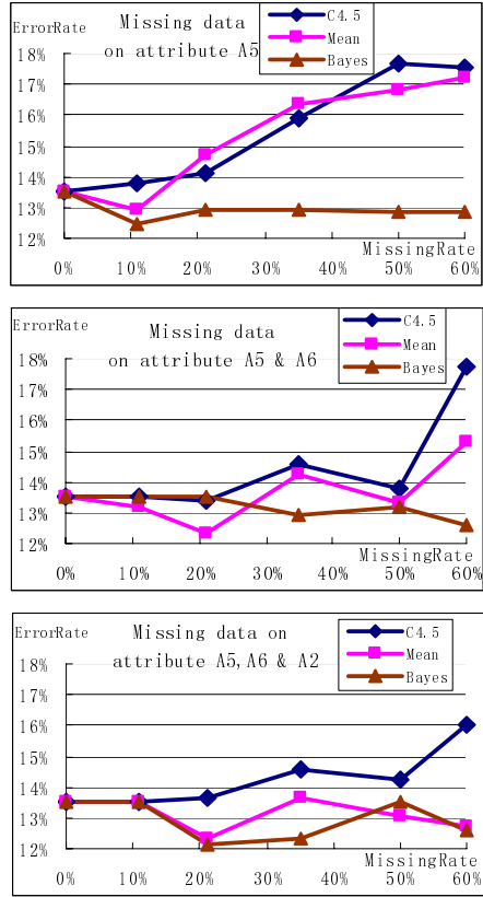
Fig. 2. Comparative results for Crx
