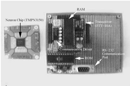
Fig. 2. Neuron device and implemented BLN board
