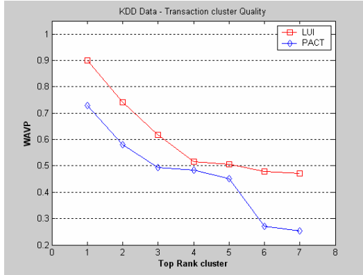
Fig. 3. User cluster quality analysis results upon WAVP comparison for KDD dataset
