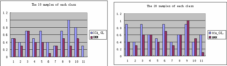
Fig. 4. (Left) Result compare with ICA_GL and HMM in the 10 samples of each class (Right) Result compare with ICA_GL and HMM in the 20 samples of each class
