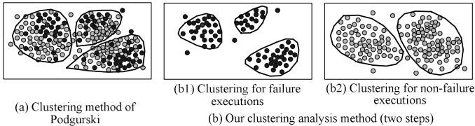
Fig. 3. An exhibitive diagram of two clustering methods. The gray points represent non-failure executions, and black points represent the failure executions. The distances between the points approximate the dissimilarities. Note that the distributions of points' positions are different between (a) and (b), because we adopt another dissimilarity measure compared with Podgurski's
