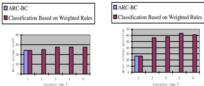
Fig. 3. Micro-Average-Recall and Micro-Average-Precision on the Open Testing
