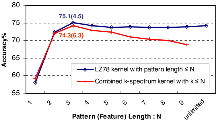
Fig. 3. Peaking of classification or finite sample size effect for melody classifier. The performance with feature size close to the optimal point D(3) are shown in the figure
