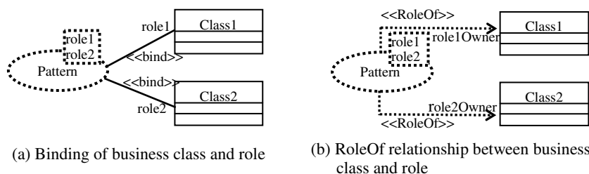
Fig. 1. Design pattern instantiation
