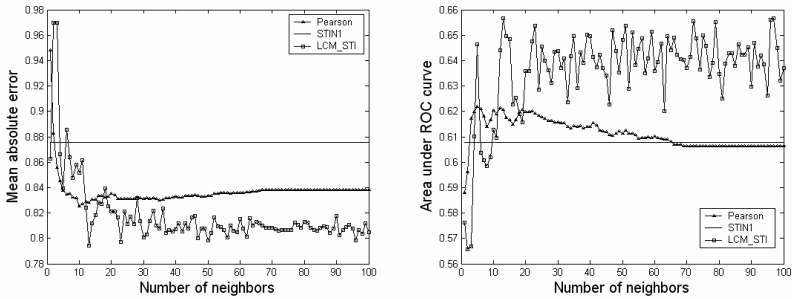
Fig. 1. The prediction results of the EachMovie dataset: MAE ( left ) and ROC ( right )
