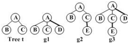
Fig. 3. A free tree t has two extension points ‘A’ and ‘C’ and two extensions containing (A:D) and (C:E)
