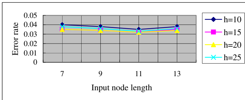
Fig. 3. The error rate curve (Hidden node number k=10, 15, 20, 25 )
