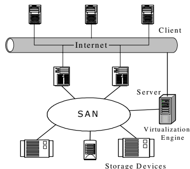
Fig. 1. The architecture of an out-of-band virtualized SAN
