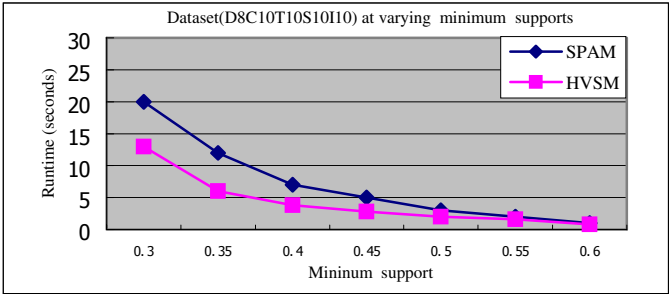
Fig. 5. Varying support for medium-sized dataset
