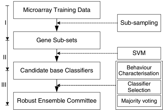
Fig. 2. The proposed ensemble learning approach
